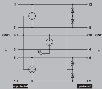
Complete module, indirect earthing
