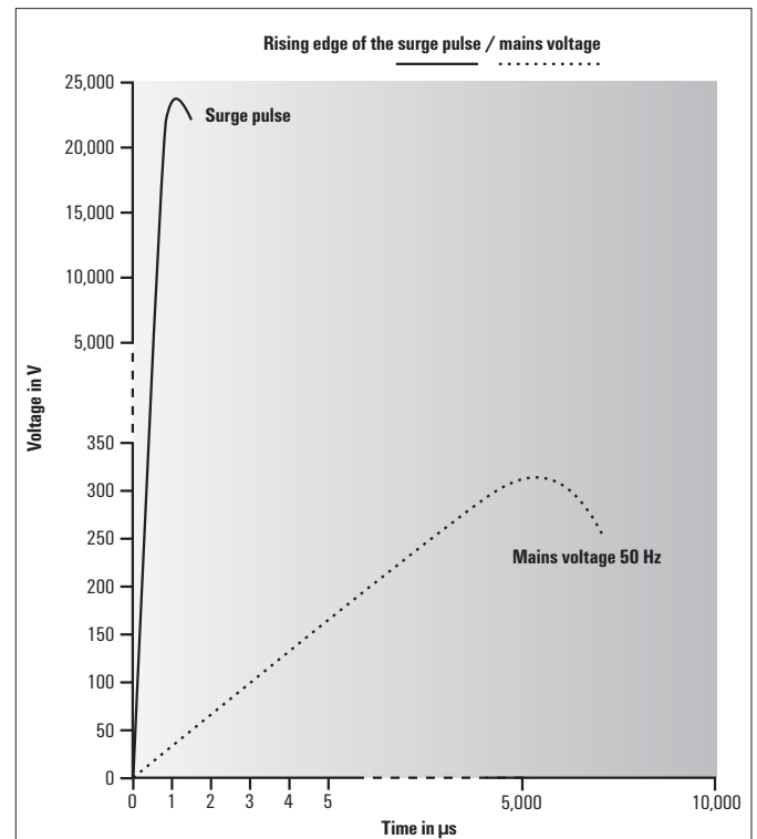
Edge behaviour between a 50 Hz sine wave and surge pulse
