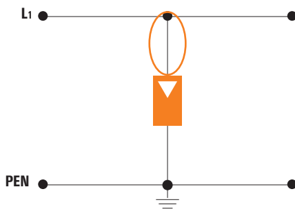
Line conductor wiring
