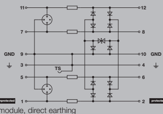
Complete module, direct earthing
