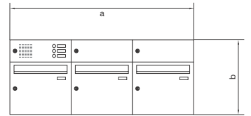
EAT-x/x a = 435 mm b = 515 mm Tiefe = 10 mm Edelstahl
