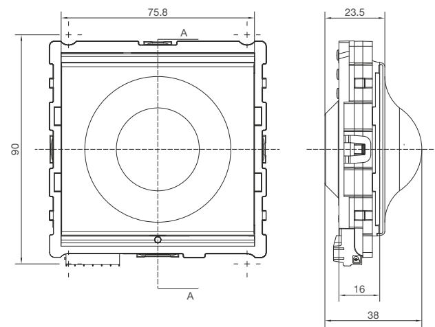
Video-Modul EB 2Draht REU610Y
